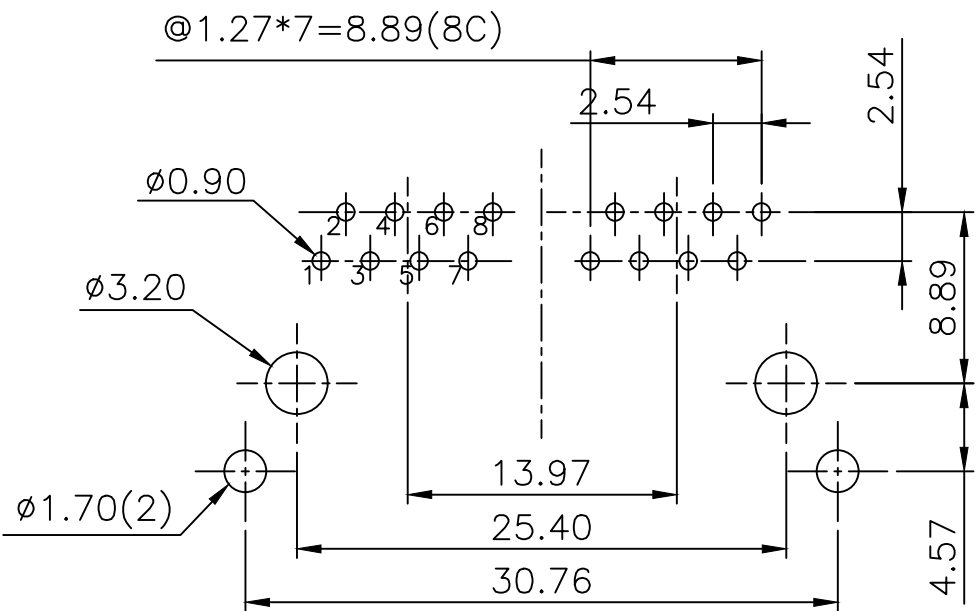
PC Board Layout Component Side Shown
